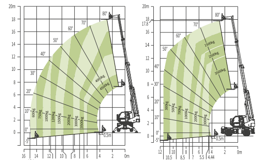
Range of Motion ZTH4518R
