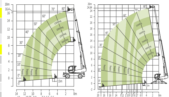
Range of Motion ZTH4525R
